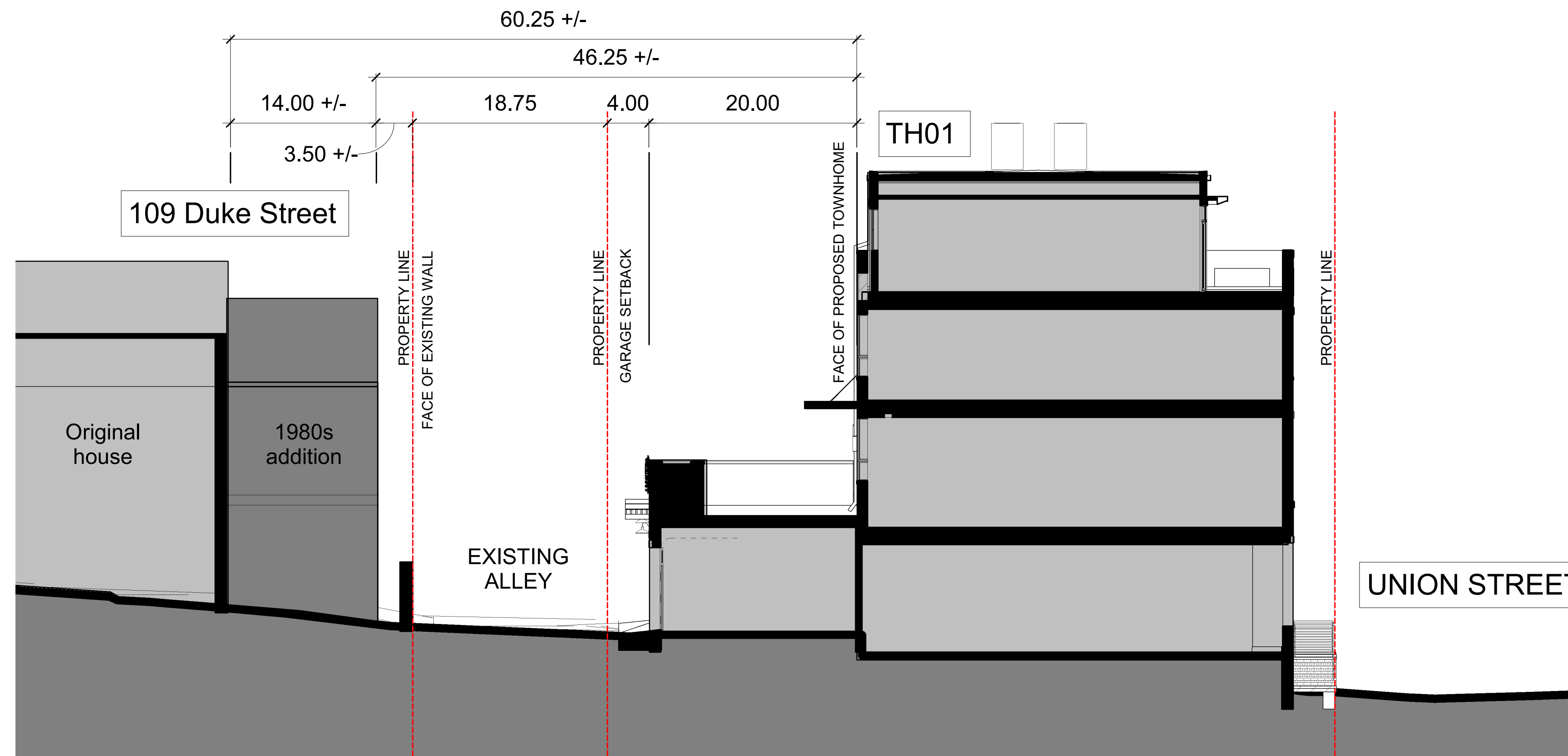
1 SECTION AT ALLEY WITH 109 AND 101 DUKE STREET 1/8" = 1'-0"
