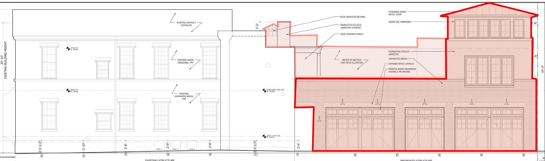
Alley (north) Elevation
