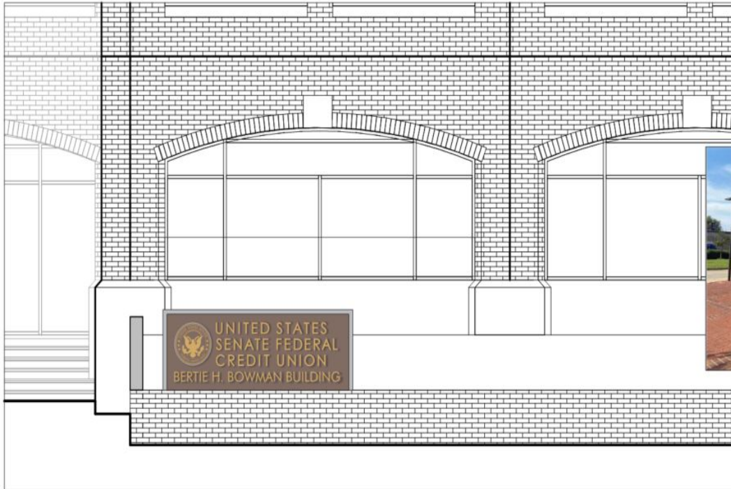
1 PARTIAL SOUTH ELEVATION VIEW SCALE: 1/4" = 1'-0"
