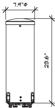
CYLINDRICAL ANTENNA
