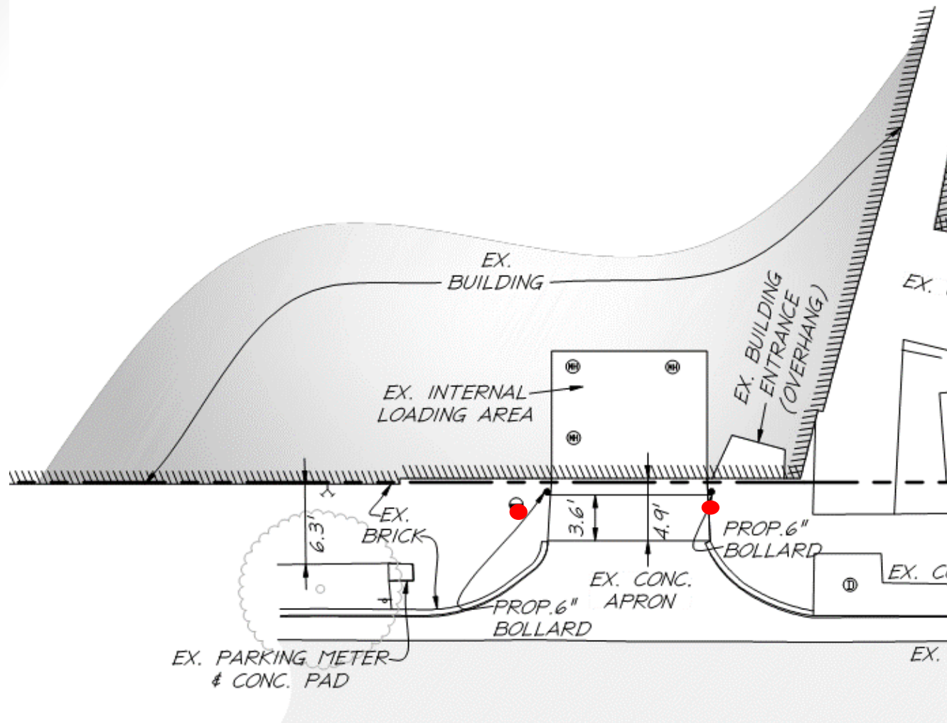
Figure 2: Indicates proposed bollards
