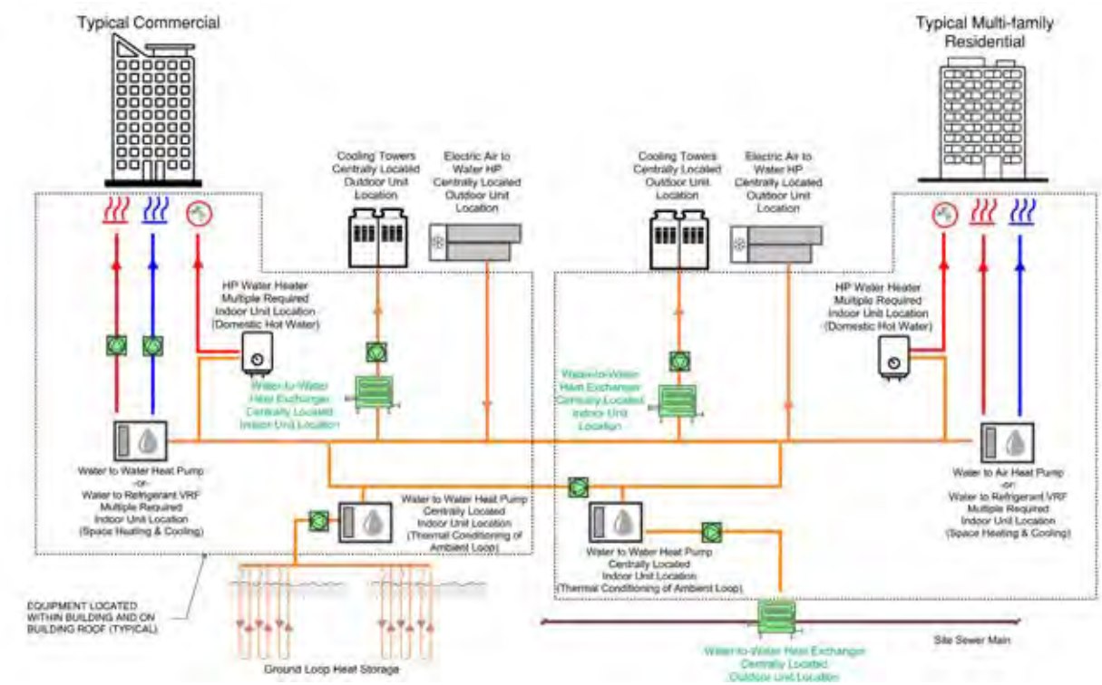
SCENARIO 4: CW + AMBIENT LOOP + GEOTHERMAL HEAT PUMP + SEWER HEAT
