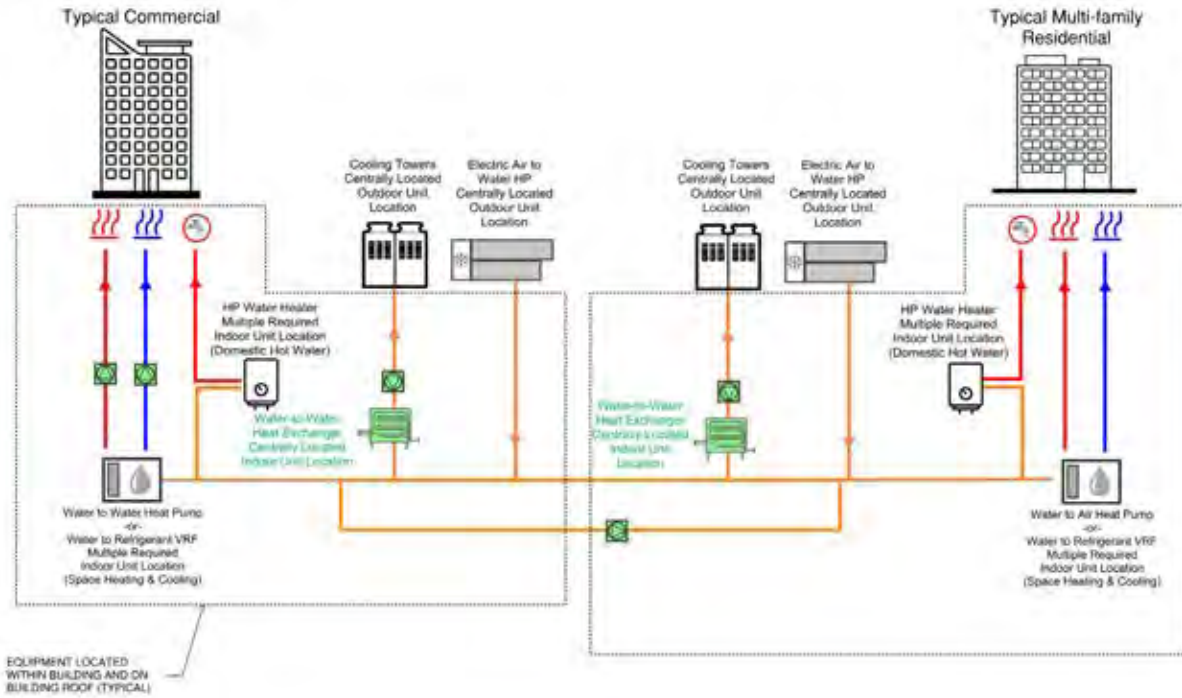
SCENARIO 1: CW+ AMBIENT LOOP
