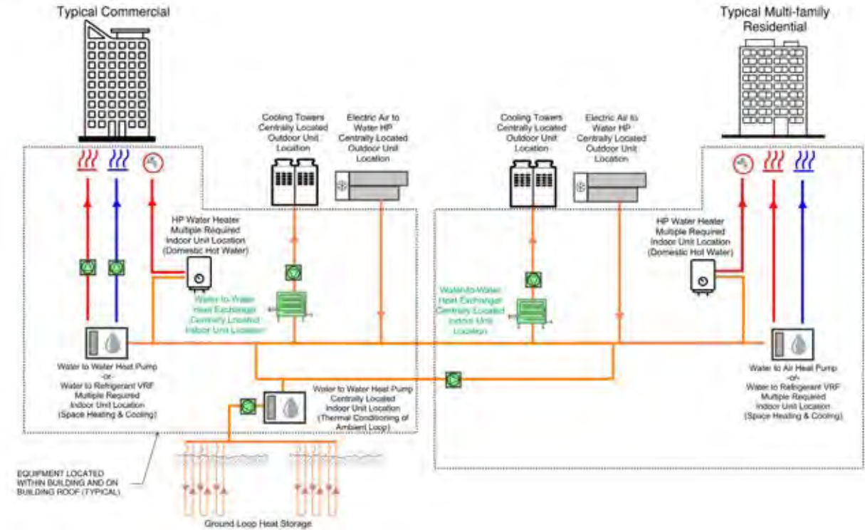
SCENARIO 2: CW + AMBIENT LOOP + GEOTHERMAL HEAT
