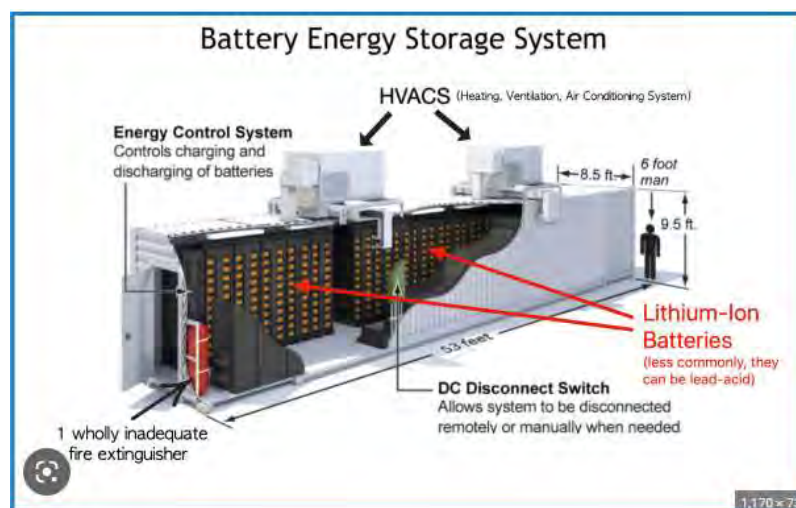
Figure 2. BESS Example
