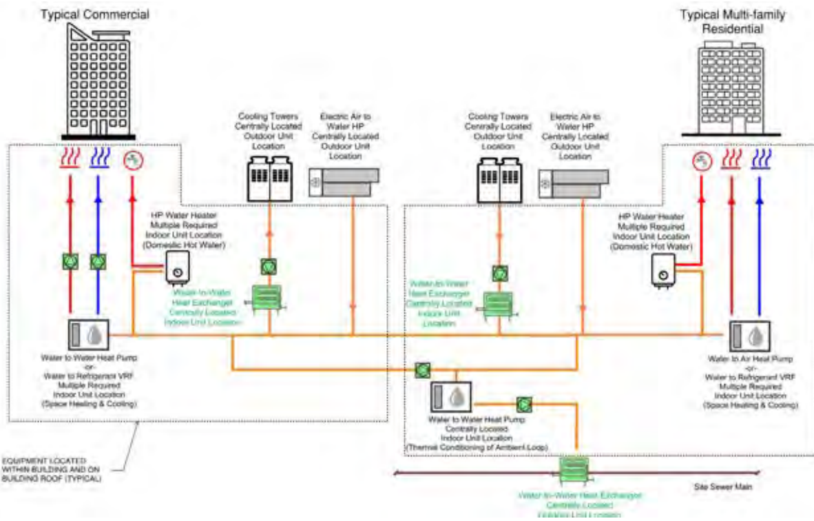
SCENARIO 3: CW + AMBIENT LOOP + SEWER HEAT
