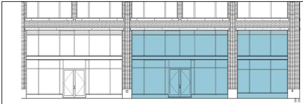
District Dogs South Elevation
