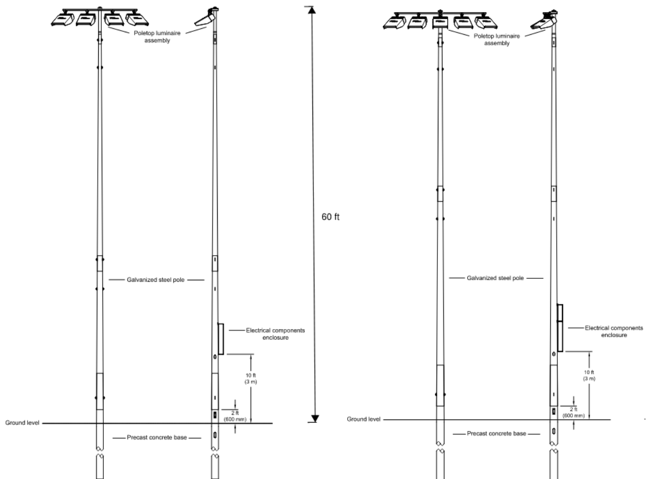
Graphic 1 – Elevations of two types of Light Poles proposed
