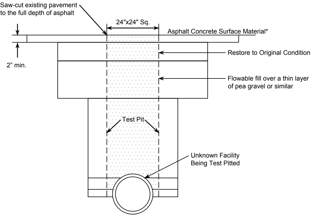
ASPHALT RESTORATION TEST PIT DETAIL SQUARE TEST PIT
