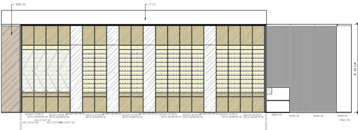
6 EL2 INTERIOR ELEVATION SCALE: 1/4" = 1'-0"
