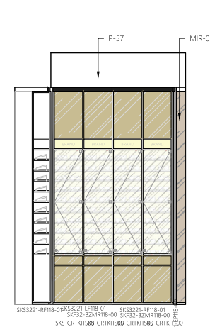
5 EL1 INTERIOR ELEVATION SCALE: 1/4" = 1'-0"
