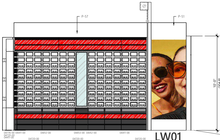
2 EL1 INTERIOR ELEVATION SCALE: 1/4" = 1'-0"
