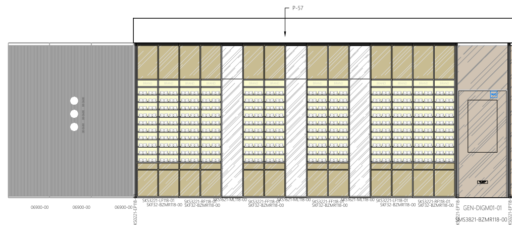
8 EL2 INTERIOR ELEVATION SCALE: 1/4" = 1'-0"
