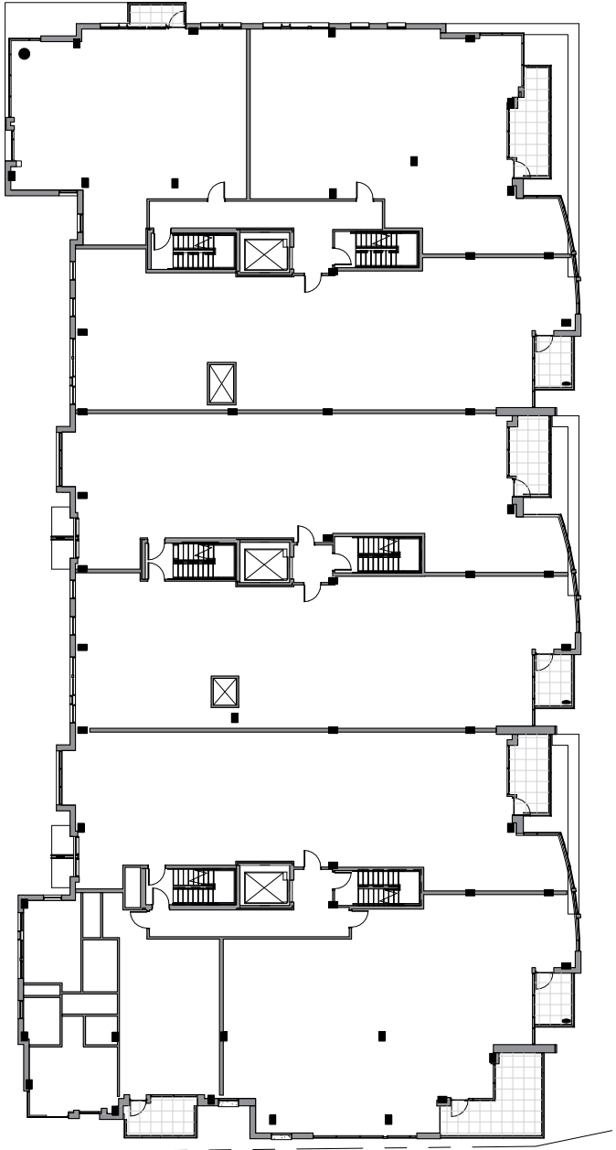
SECOND/THIRD FLOOR PLAN
