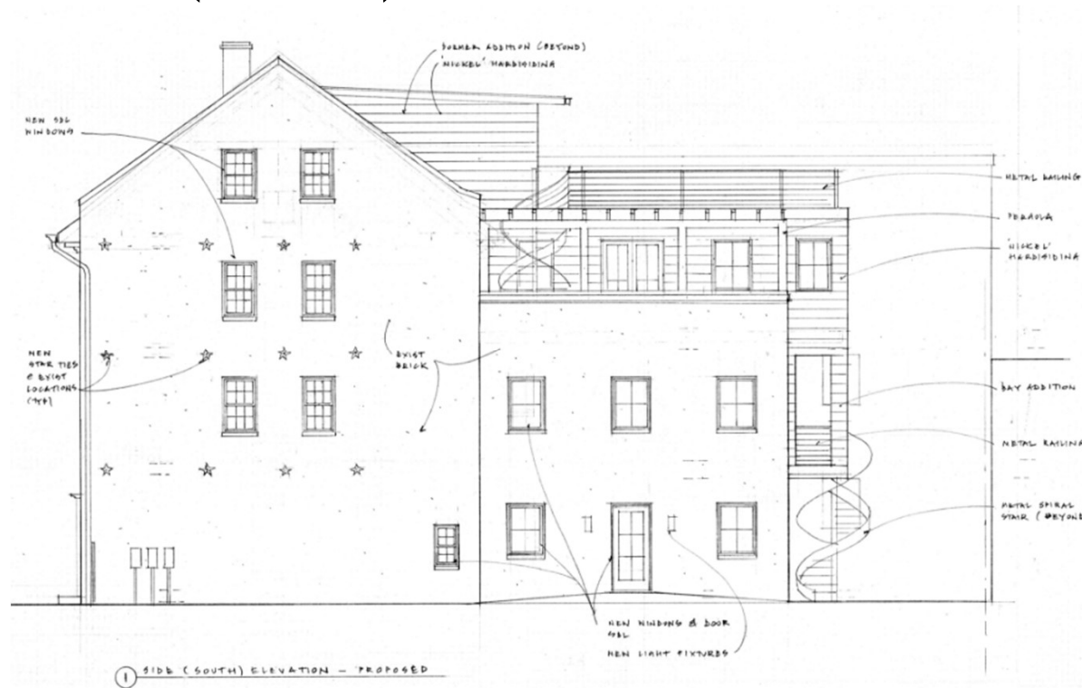
Proposed side (south) elevation
