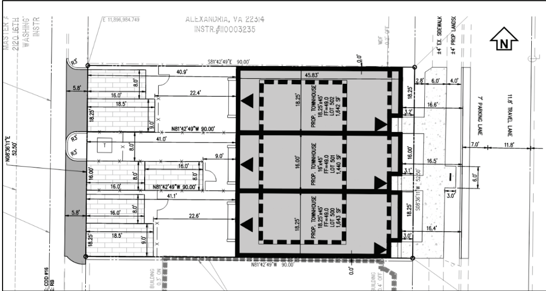
Figure 4: Site plan
