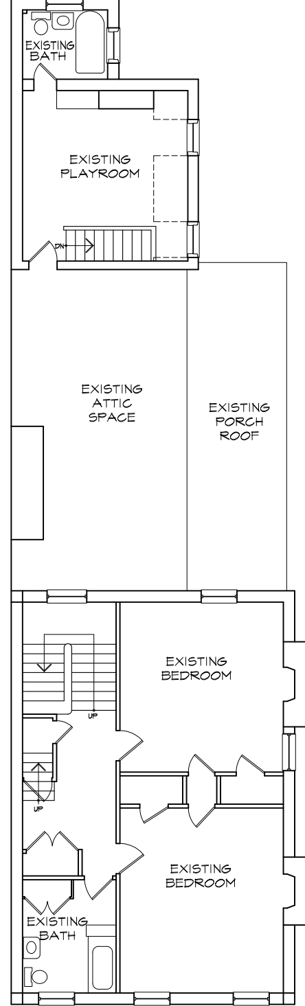
EXISTING THIRD FLOOR PLAN 1/4"=1'-0"
