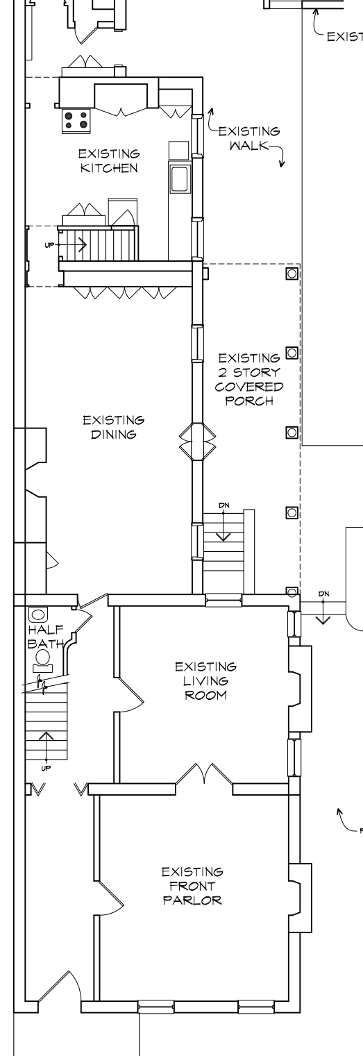
EXISTING FIRST FLOOR PLAN 1/4"=1'-0"
