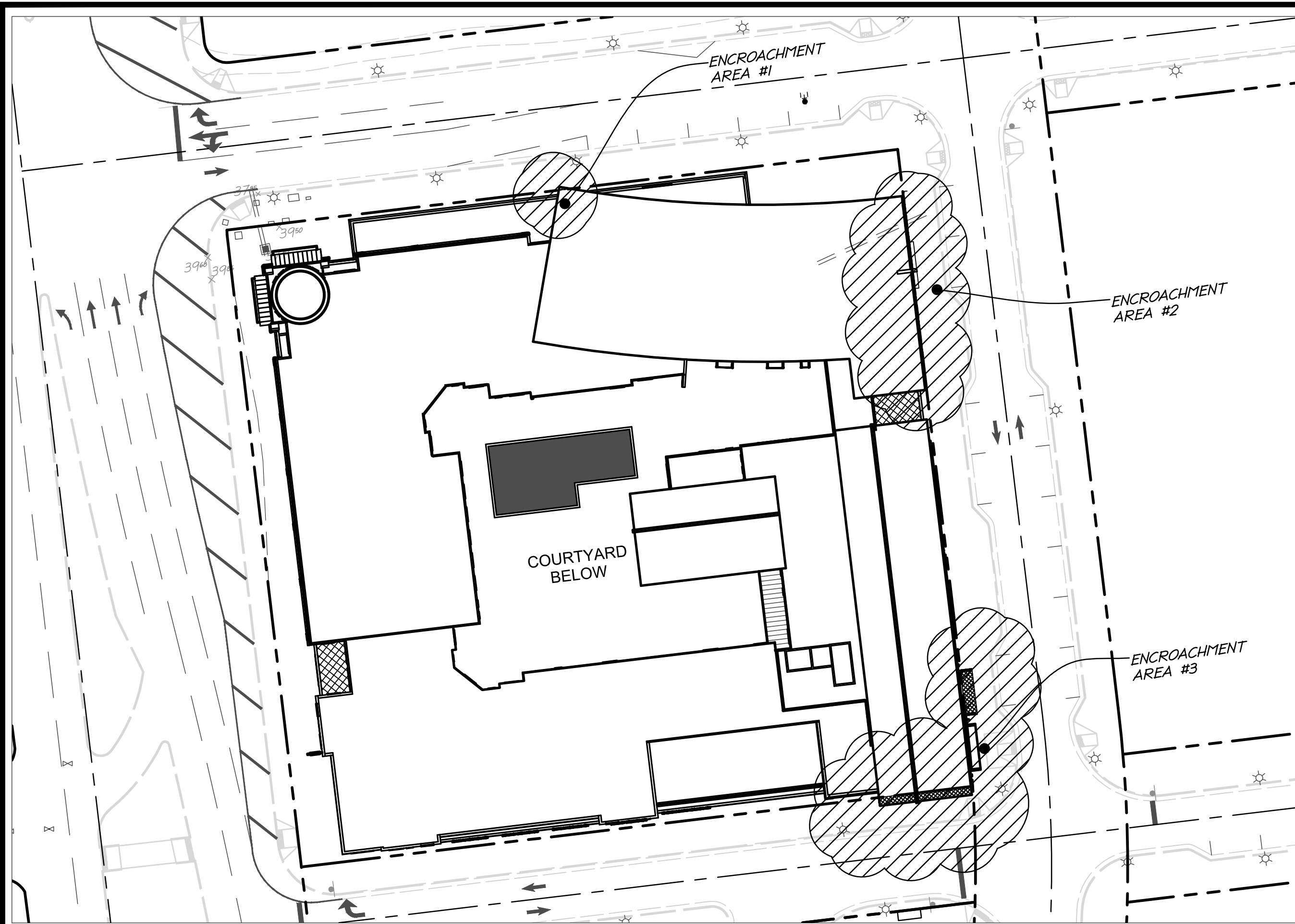
BLOCK H - OVERALL (1"=40')
