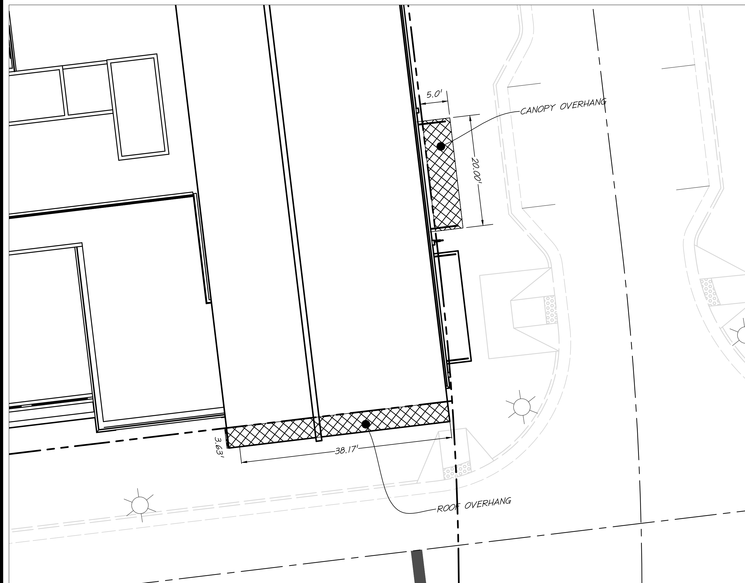
BLOCK H - ENCROACHMENT AREA 3 (1"=10')
