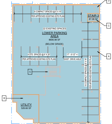
LOWER PARKING LEVEL 1 1/16" = 1'-0" DETAIL
