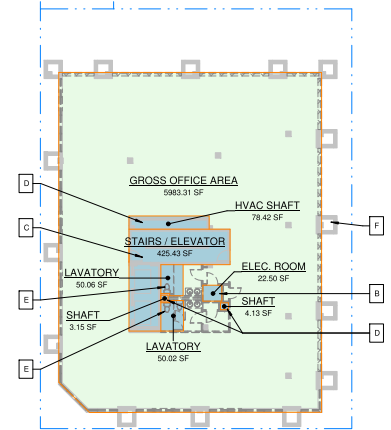
LEVEL 3 5 1/16" = 1'-0" DETAIL
