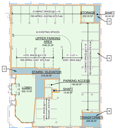
LOBBY LEVEL 3 1/16" = 1'-0" DETAIL
