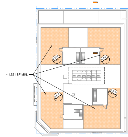
ROOF OPEN SPACE 3 1/16" = 1'-0"
