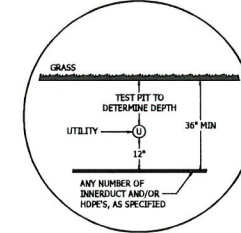
UTILITY CROSSING (GRASS) SCALE: NTS
