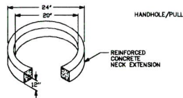
TYPICAL DETAIL "D"
