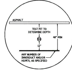
STORM DRAIN CROSSING (ASPHALT) SCALE: NTS
