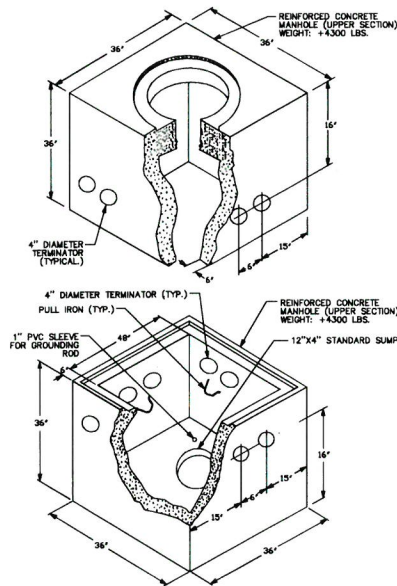
TYPICAL DETAIL "D"
