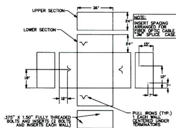
TYPICAL DETAIL "F"
