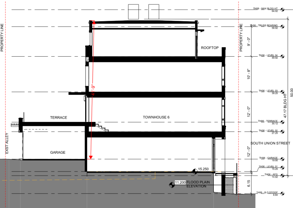
2 TH06 GRADING SECTION. 1/8" = 1'-0"
