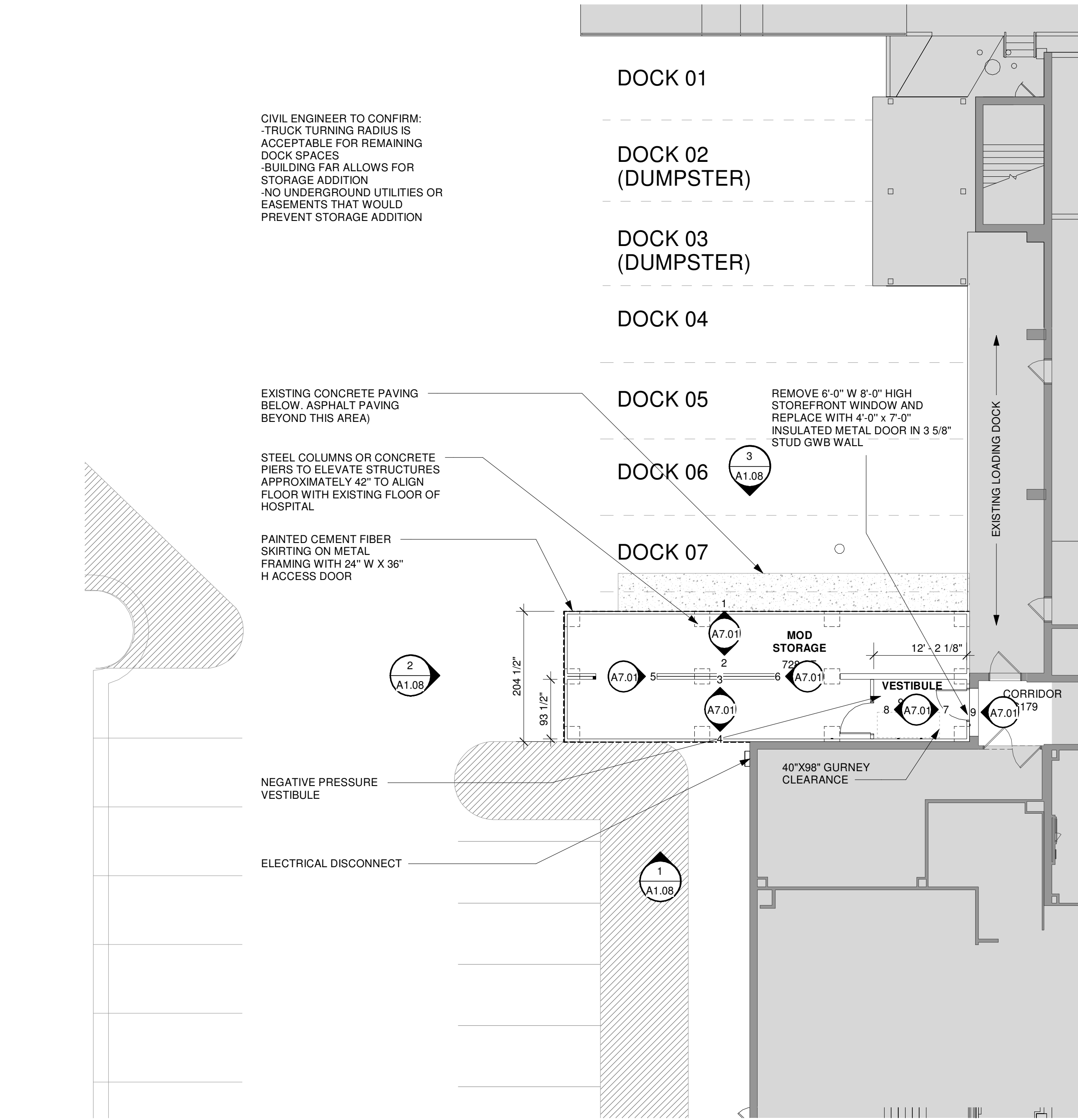
2 ENLARGED SITE PLAN - NEW WORK 3/32" = 1'-0"
