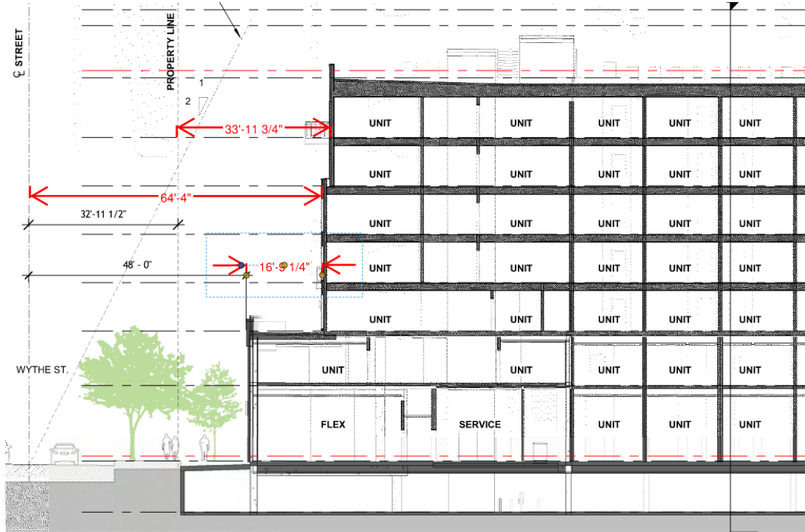
Figure 1: Wythe Street Building Setbacks
