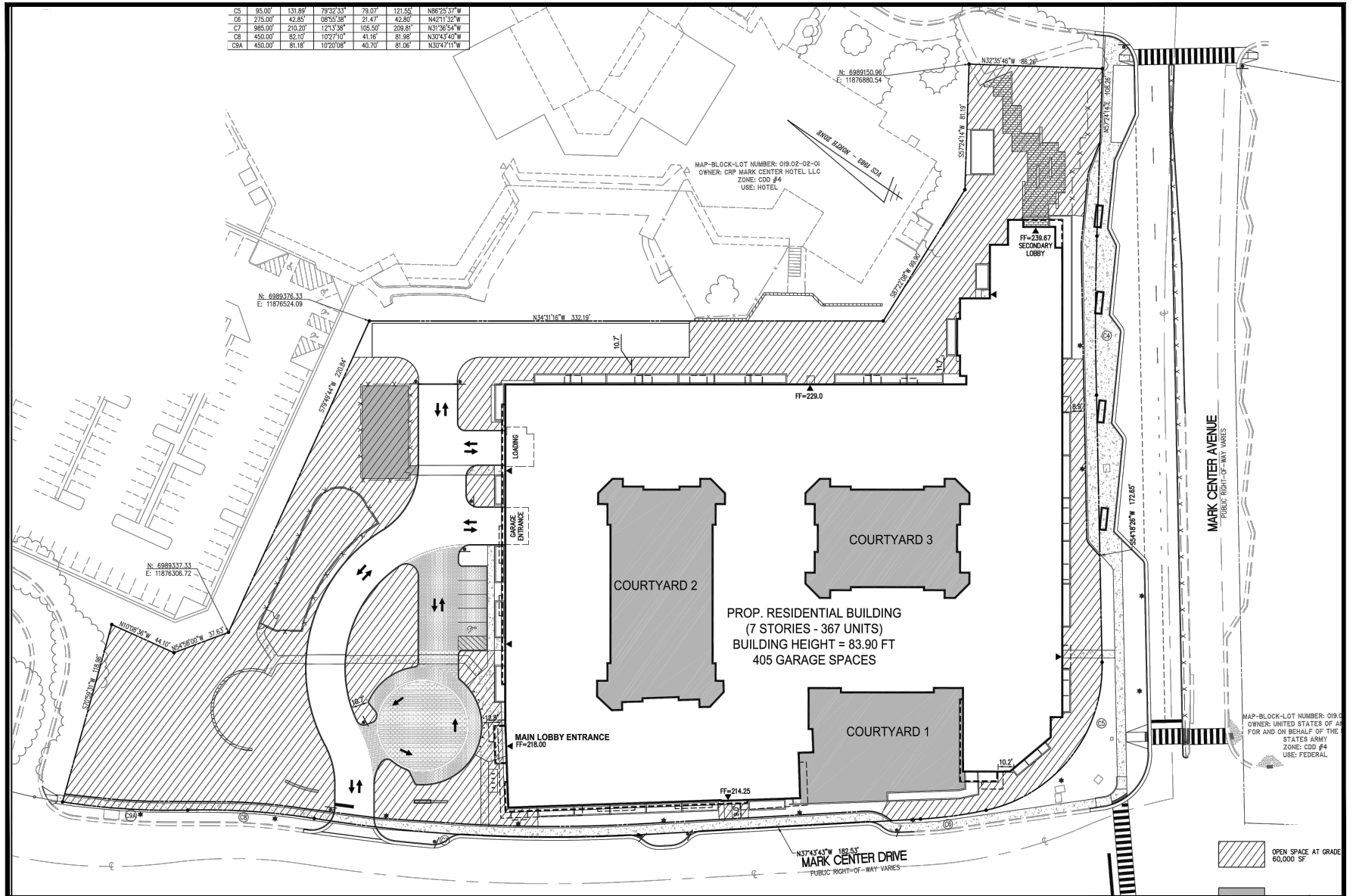
Figure 2-2 Site Plan
