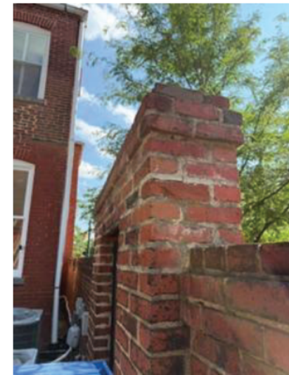
Detail of brick ornamental cap on wall and archway (1 cap bricks in line with wall plane, with 2 rows of cantilevered bricks below)
