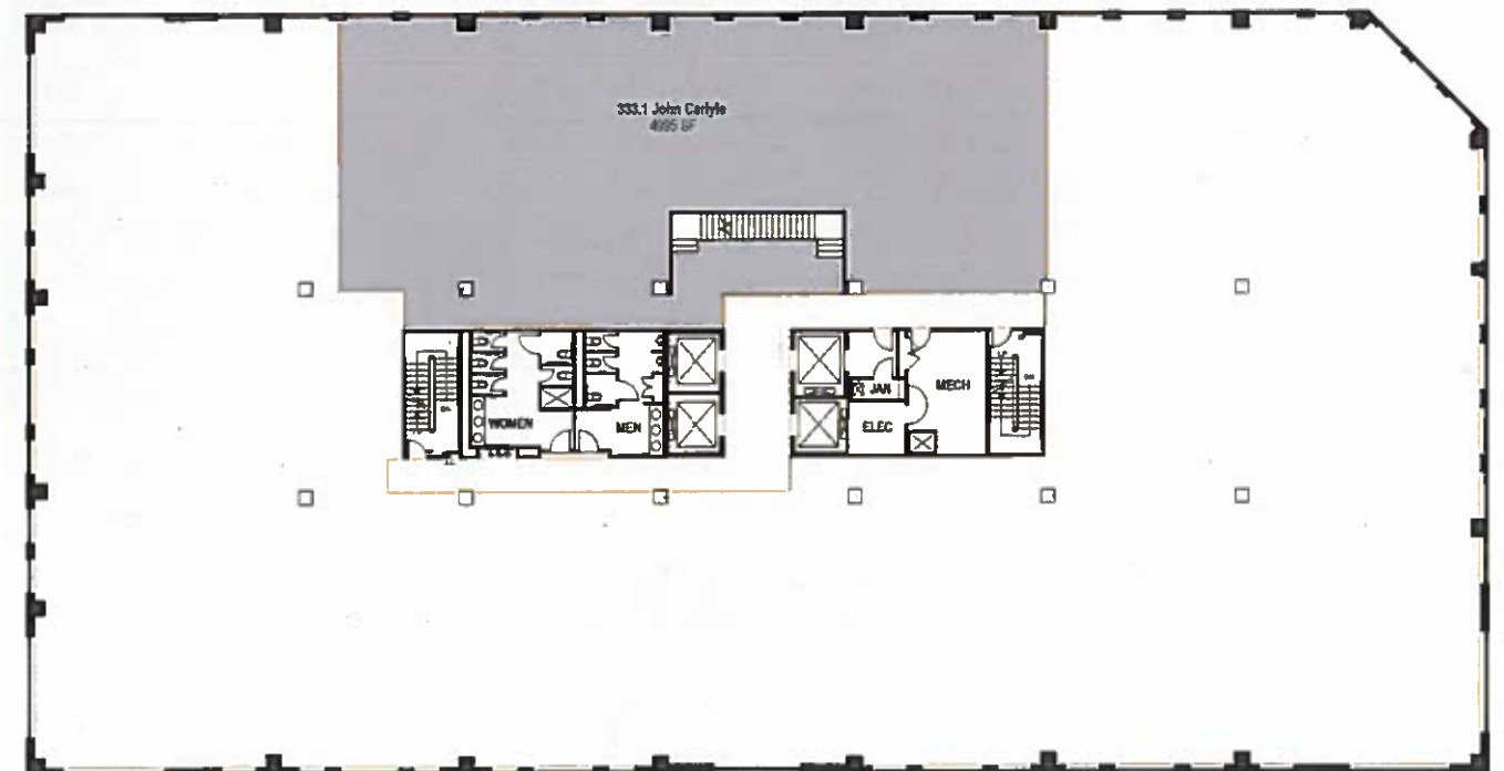
04 LIFE SAFETY PLAN - LEVEL 04 - 333.1 John Carlyle SCALE: 1/16" = 1'-0"
